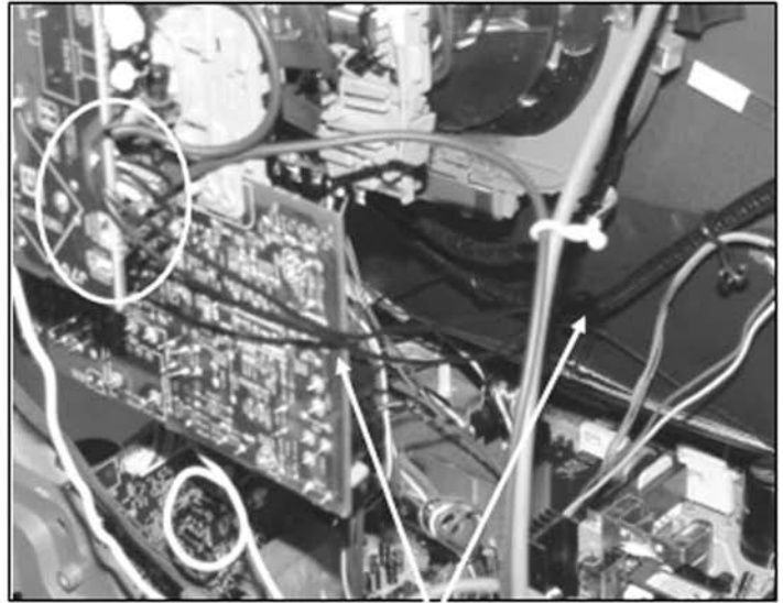
Dress CRT ground wires behind DGC and beside VD board
