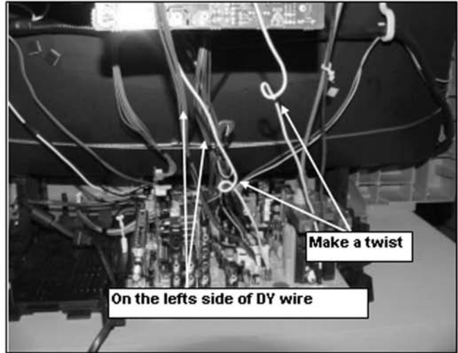
Dress G2 wire and DF wire as shown in picture. Dress heaters and VM harnesses on the left side of DY lead wire
