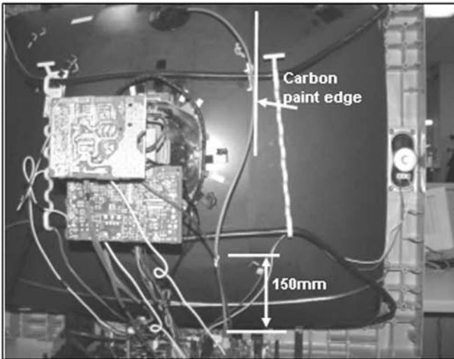
Dress HV cable and focus wire together using a 5mm purse lock, install purse lock 150mm±10 from rubber cap . Dress HV through standing holder, install holder on CRT's carbon paint edge
