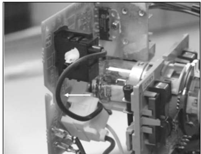
Bend H-Stat wire towards C board.
