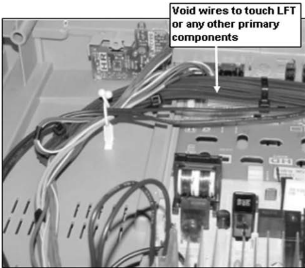
Dress HM board grounding wires, HR harness and HU 12P harness together into standing purse lock, dress 12P YUV harness (M-HM board) with DGC tube behind purse lock and under 6P HR and 12P HU harnesses.
