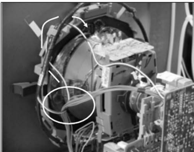
Dress RGB harness over Rotation coil lead wire. Dress Rotation coil lead wire over DY clip and through rotation coil as shown in picture.
