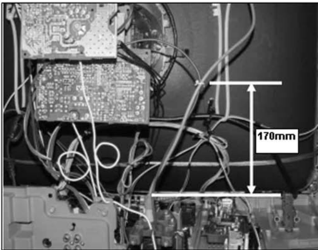
Dress HV and focus lead wire together using a 5 mm purple lock (3-703-981-02) as shown in picture.
