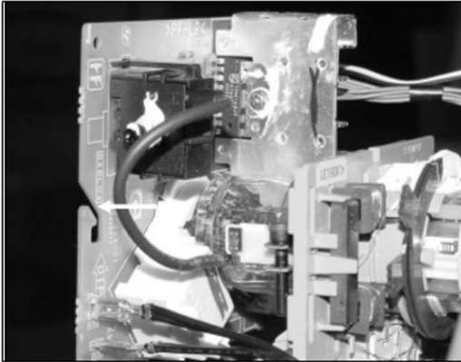
Bend H-Stat wire towards C board.
