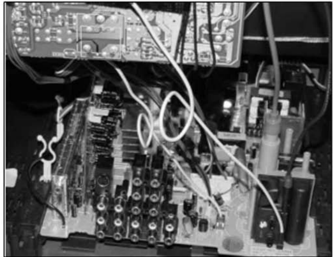
Dress G2 wire and DF wire as shown in picture.
