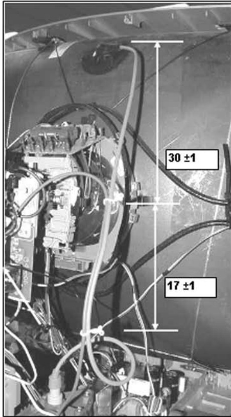
Dress together focus lead and HV cable using (2) 5mm (3-703-981-02)
