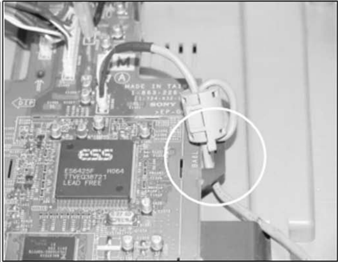
Dress 3P connector from HM~HN board through hook as in picture. Install ferrite 60mm from housing
