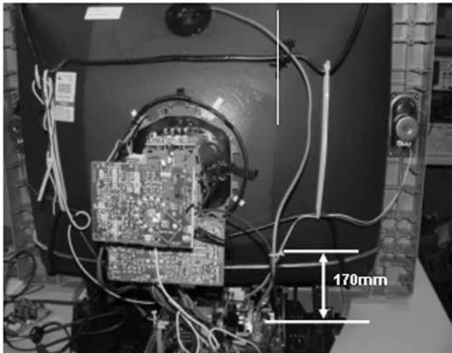
Dress HV cable and focus wire together using a 5mm purse lock (3-703-981-02). Install purse lock over carbon paint edge.
