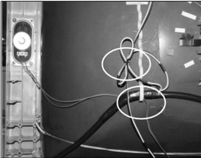
Dress right speaker wire through DGC band. Dress DGC lead wire with a 9mm purse lock
