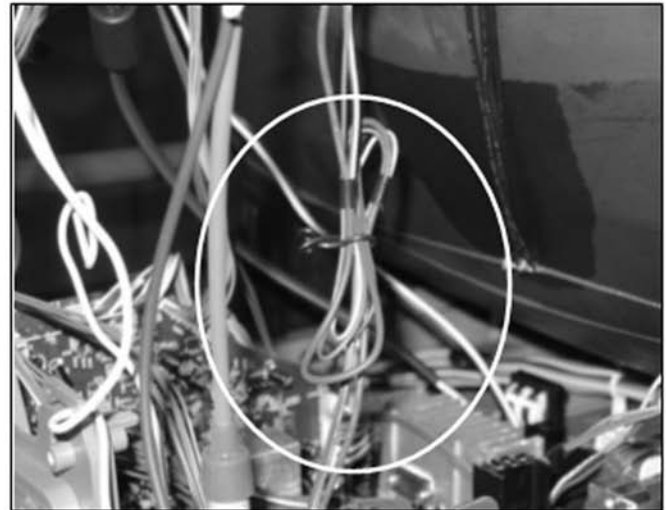
Dress DY lead wire with a 9mm purple lock (3-703-982-02)
