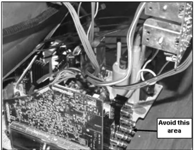
Dress VM and heaters harnesses over RGB to avoid interference with back cover installation.
