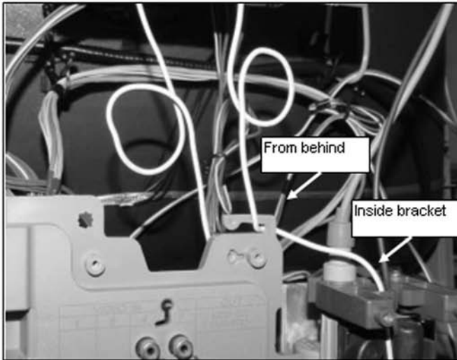
Dress G2 wire inside FBT bracket, behind A/V bracket hook (from behind) and make a loop. Dress DFT wire making a loop.
