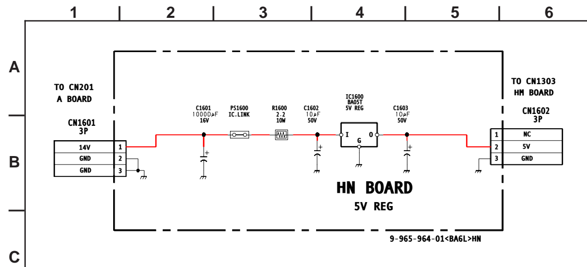
HN BOARD SCHEMATIC DIAGRAM (KV-27FS320/32FS320/36FS320 ONLY)
