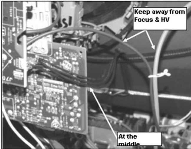
Dress CRT ground wires under DGC and beside VD board at the middle as picture shows, keep away from focus and HV lead wires.
